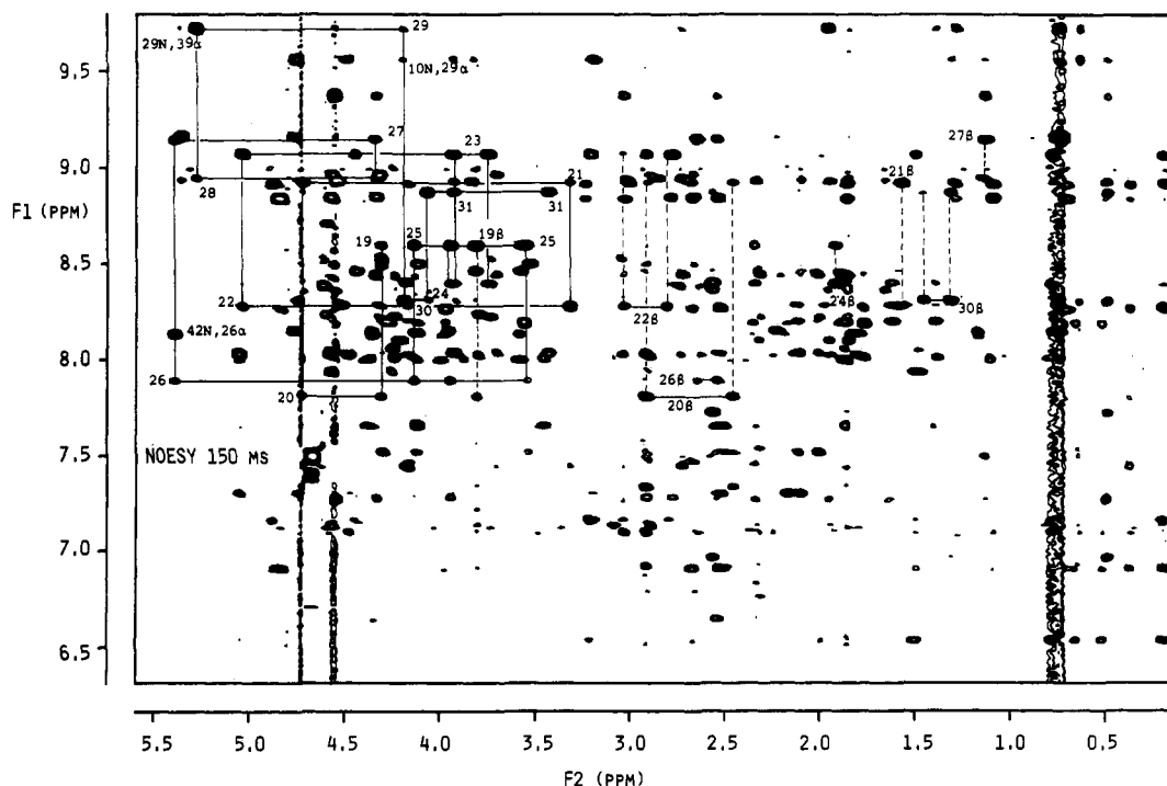
FIGURE 4: NH/aromatic(F1-axis)-aliphatic(F2-axis) region of the 150-ms NOESY spectrum of hirudin in H 2 O. The sequence of d_{\alpha N}(i, i + 1) connectivities extending from residue 19 to residue 31 is indicated by a continuous line, and the peaks are labeled at the positions of the intraresidue NH(i)-C α H(i) cross peaks. Some d_{\beta N}(i, i + 1) connectivities are indicated by dashed lines. Also labeled are a few long-range NH-C α H connectivities. The spectrum is unsymmetrized and was recorded by using the semiselective jump-return sequence for the last 90° pulse to suppress the water resonance.
