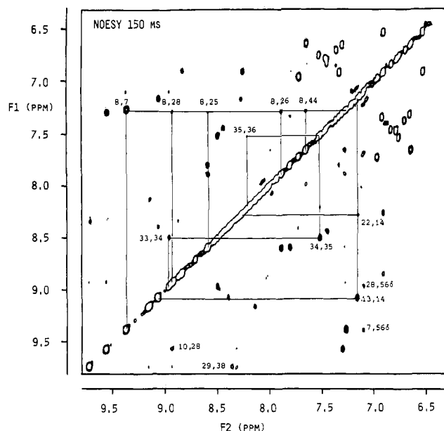
FIGURE 3: NH(F1-axis)-NH(F2-axis) region of the 150-ms NOESY spectrum of hirudin in H 2 O. The sequence of d_{NN}(i, i + 1) connectivities extending from residue 33 to residue 36 as well as that of some long-range d_{NN} connectivities is indicated. The spectrum is unsymmetrized and was recorded by using the semiselective jump-return sequence for the last 90° pulse to suppress the water resonance.
