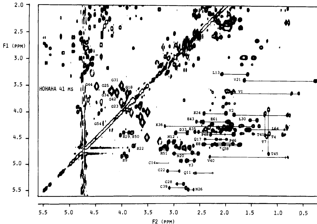
FIGURE 2: A portion of the C ^{\alpha} H(F1-axis)-aliphatic(F2-axis) region of the HOHAHA spectrum of hirudin in D_2O . Direct and relayed connectivities are present, and some spin networks originating from the C ^{\alpha} H protons are indicated by continuous lines. The spectrum is unsymmetrized.
