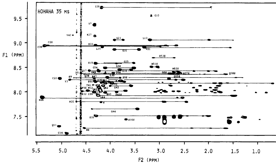
FIGURE 1: NH(F1-axis)-aliphatic(F2-axis) region of the HOHAHA spectrum of hirudin in H_2O . Some relayed connectivities are indicated by continuous lines, and the labels are at the positions of the direct NH-C ^{\alpha} H cross peaks except where indicated. The spectrum is unsymmetrized. Note that, in a few cases involving C ^{\alpha} H protons located directly under the water resonance such that the NH-C ^{\alpha} H cross peaks are no longer observable, the corresponding relayed cross peaks to the C ^{\beta} H protons are still apparent (e.g., N37, T5, D52, and D55). In this portion of the spectrum the NH-C ^{\alpha} H cross peaks of T4 and C6 (8.92, 4.63 and 8.90, 4.59 ppm), which are located just to the high field of the water resonance, are not visible and no associated relayed peaks could be observed; these NH-C ^{\alpha} H cross peaks, however, could be detected in the symmetrically related region of the HOHAHA spectrum. The three peaks marked x do not arise from native hirudin. They probably arise from the population of minor hirudin variants present (see Experimental Procedures).
