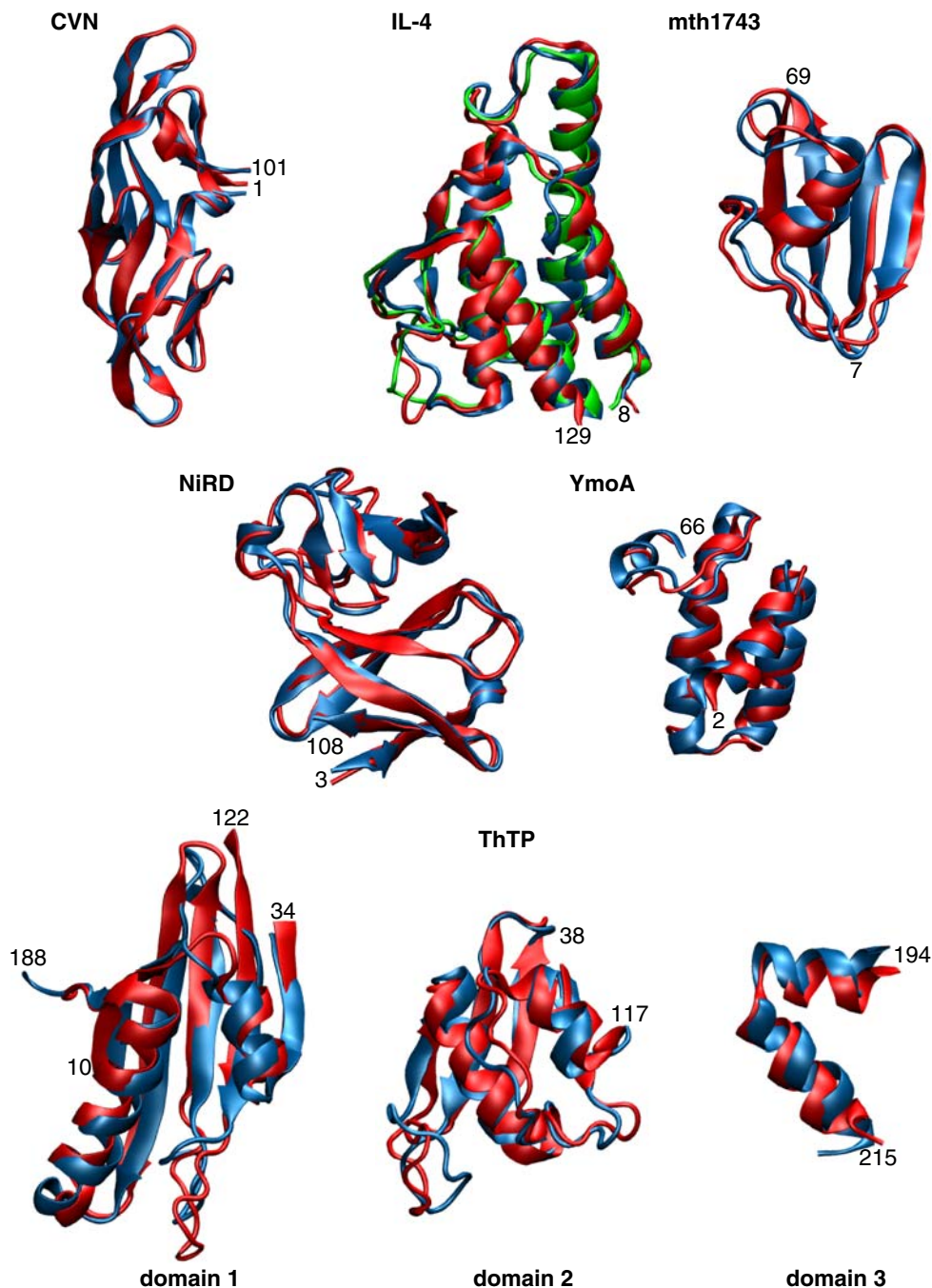
Fig. 3 Results of the PASD algorithm for six proteins. Reference NMR structures are drawn in red. The reference X-ray structure of IL-4 is drawn in green. The regularized mean coordinates of the converged second-pass PASD structures are drawn in blue. ThTP consists of three domains whose relative orientations were not determined, but the individual domains were solved, as shown. Termini of the defined regions (see Table 3) are labeled
