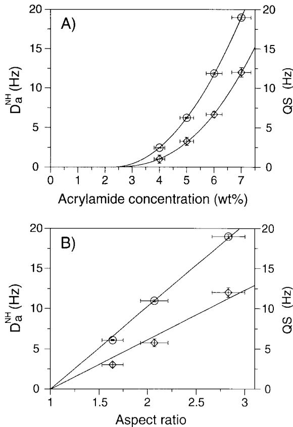
Figure 3. Dependence of G/B1 alignment tensor magnitude ( \circ ) and solvent ^2\text{H} quadrupolar splitting ( \diamond ) on (A) acrylamide concentration and (B) the aspect ratio of the compressed gel, (d_o/d_N)^3 . The curves drawn in (A) correspond to D_a^{NH} = 0.87 \times (c-2.3)^2 and QS = 0.29 \times (c-2.3)^{2.4} , for d_o/d_N = 1.42 . The straight lines in (B) correspond to D_a^{NH} = 10.3 \times [(d_o/d_N)^3 - 1] , and QS = 6.2 \times [(d_o/d_N)^3 - 1] , for an acrylamide concentration of 7%.
