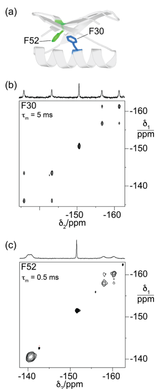
Figure 5. Ring flips of \text{F}_3\text{Phe} in positions 30 or 52 of GB1 are in the slow exchange regime at 25 °C. (a) Structure of GB1 (PDB ID 2QMT) 41 showing the sites of the \text{F}_3\text{Phe} mutations. (b) [\text{F}_3, \text{F}_3]\text{-NOESY} spectrum of \text{F}_3\text{Phe} in position 30. The mixing time is indicated in the spectrum and the 1D ^{19}\text{F} NMR spectrum is shown above. (c) Same as (b) but for position 52. Narrow signals at -142.6 , -156.0 , and -162.5 ppm correspond to traces of denatured protein.
