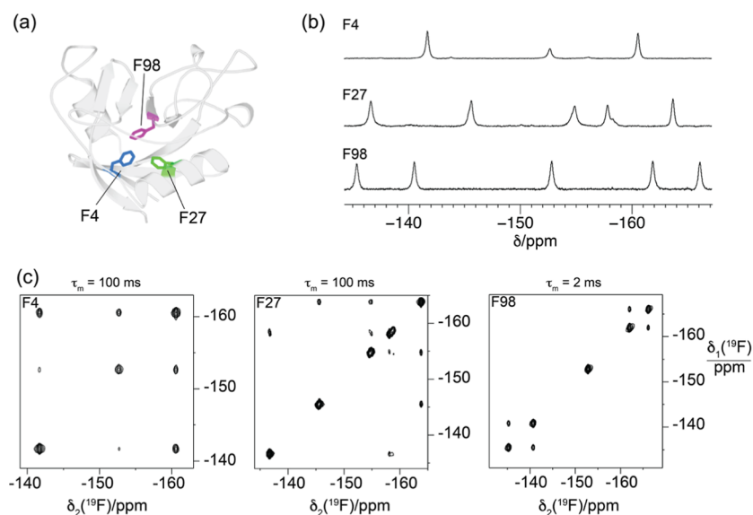
Figure 4. ^{19}\text{F} NMR spectra of PpiB with \text{F}_3\text{Phe} replacing F4, F27, or F98. (a) Structure showing the sites of the \text{F}_3\text{Phe} mutations. (b) 1D ^{19}\text{F} NMR spectra recorded at 25 °C on a 600 MHz NMR spectrometer and processed with 10 Hz line broadening (c) [\text{F}_3, \text{F}_3]\text{-NOESY} spectra recorded on a 400 MHz NMR spectrometer. The spectra are annotated with the mixing time used and the site of \text{F}_3\text{Phe} incorporation. Acquisition parameters are provided in Table S4.
