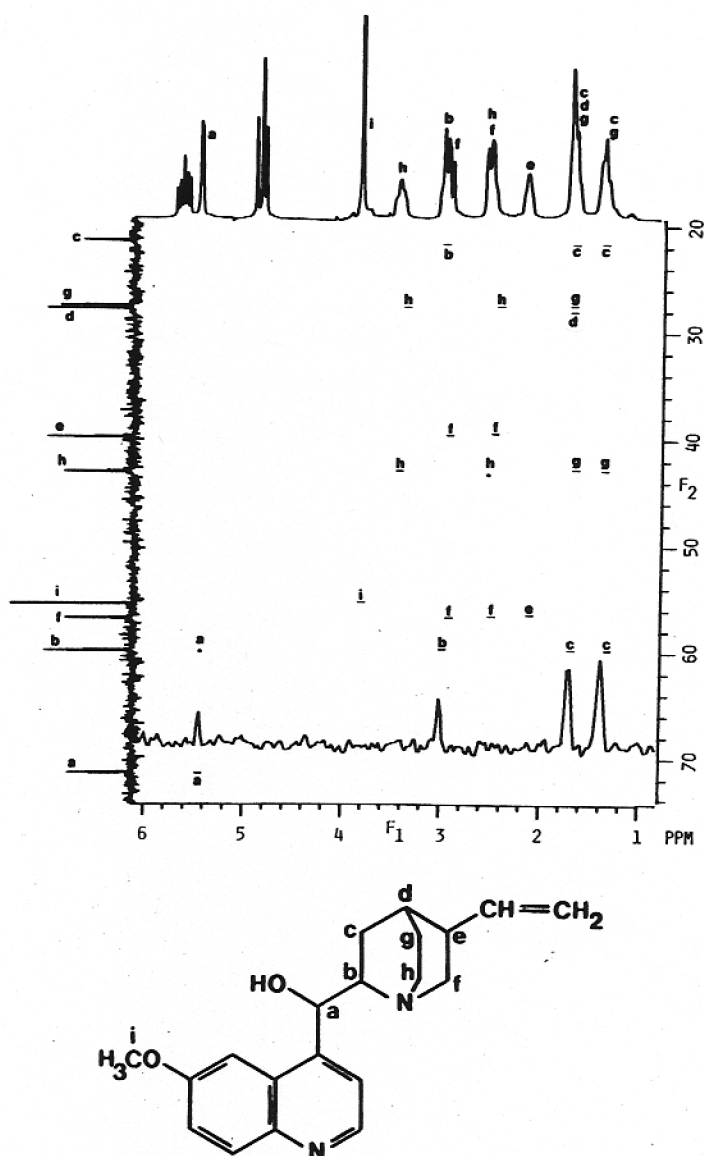
FIG. 2. Heteronuclear RELAY spectrum of quinine, recorded on a 270 MHz spectrometer. The assignment of the carbons is indicated on the spectrum along the vertical axis. In the 2D spectrum it is indicated from which proton the various peaks originate. For example, the peak labeled "b" at the F_2 frequency of carbon "c" indicates magnetization relay. The inset displays a section parallel to the F_1 axis, taken at the F_2 frequency of carbon "b," showing relay connectivity to protons "c" and "a."
