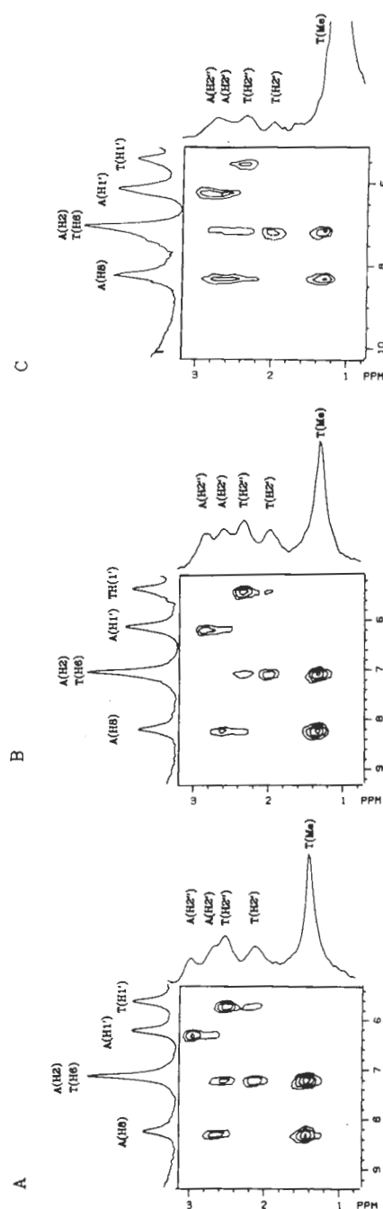
Fig. 2. Expansion of a portion of the 2D-NOE spectra of Fig. 1 showing cross-peaks for specific interactions of protons shown on one axis to the protons shown on the other axis. (A) Poly(dA-dT) · poly(dA-dT) in 0.1M NaCl, (B) poly(dA-dT) · poly(dA-dT) in 4M CsF, (C) poly(dA-dT) · poly(dA-dT) in 40% ethanol- d_6 . A mixing time of 50 ms was used in all cases.
