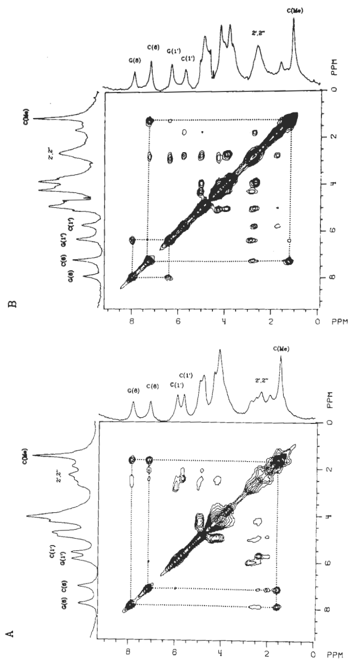
Fig. 4. Contour plots of absorption mode 2D-NOE spectra of double-stranded poly(dG-m 4 dC) in (A) 50 mM NaCl and (B) 3 mM MgCl 2 . Mixing time was 50 ms in both cases. Specific interactions are indicated by joining off-diagonal peaks for cross-relaxing protons.
