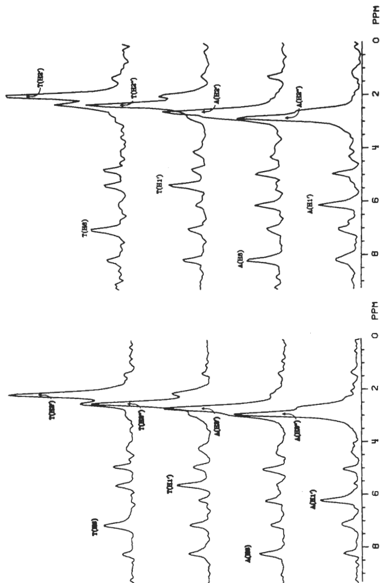
Fig. 8. Cross sections of the absorption mode 2D-NOE spectra of double-stranded poly(dA-dT) in (left) 0.1M NaCl and (right) 4M CsF with mixing times of 50 ms. See text for assignments.
