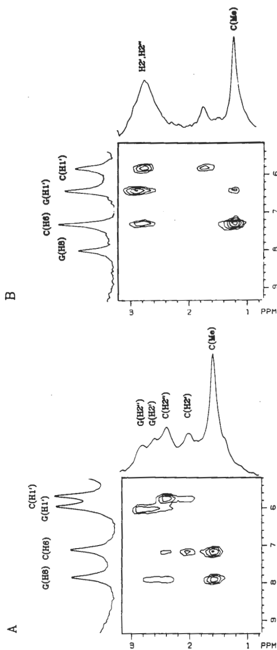
Fig. 5. Expansion of portions of the 2D-NOE spectra of Fig. 4. Cross-relaxations are indicated by cross-peaks for protons shown on one axis interacting with protons shown on the other axis. (A) Poly(dG-m 4 dC) · poly(dG-m 4 dC) in 50 mM NaCl and (B) poly(dG-m 4 dC) · poly(dG-m 4 dC) in 3 mM MgCl 2 .
