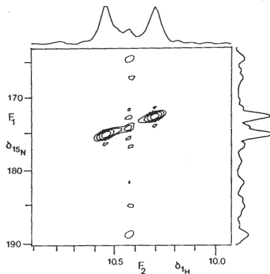
FIG. 6. Heteronuclear shift correlation spectrum obtained from the same data matrix as Fig. 5a, by using data manipulation as described in the text, to remove the proton shift contribution from the F_1 dimension. Along the F_1 and F_2 axes, the absolute value mode projections of the spectrum are shown.
