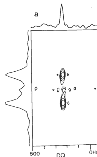
FIG. 5. (a) Heteronuclear double quantum ^{15}\text{N} concentration, obtained with The total measuring time for both mode projection of the double-quantum sections parallel to the F_1 axes, :
