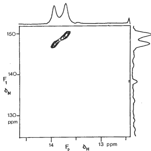
FIG. 7. ^1\text{H} - ^{15}\text{N} shift correlation spectrum of II, obtained with the sequence of Fig. 1a, and selection of the zero quantum component. Along the F_1 and F_2 axes, absolute value mode projections of the 2D spectrum are shown. The total measuring time was 2 hr.
