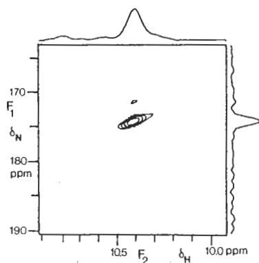
FIG. 8. Heteronuclear decoupled shift correlation spectrum of I, obtained with the sequence of Fig. 1b, selecting the double quantum signals. The total measuring time was approximately 2.5 hr. Along the two axes, the absolute value mode projections of the 2D spectrum are shown.
