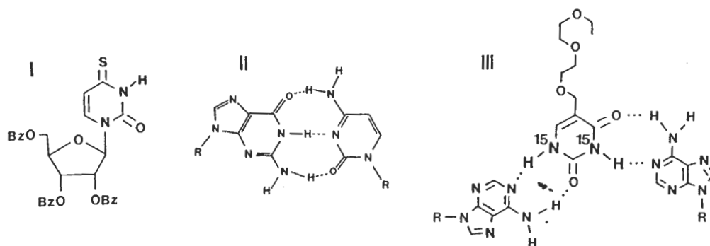
FIG. 4. Structures of 2',3',5'-tri- O -benzoyl-4-thiouridine (I), a 1:1 mixture of 2',3'- O -isopropylidene-5'- O - tert -butyldimethylsilylcytidene and 2',3'- O -isopropylidene-5'- O - tert -butyldimethylsilylguanosine (II) and a 1:2 mixture of [1,3- ^{15}\text{N}_2 ]5-(2',5',8'-trioxadecyl)uracil and 5'-acetyl-2',3'- O -isopropylideneadenosine (III).
