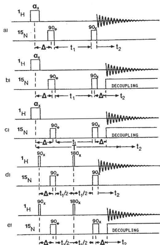
FIG. 1. Various experimental schemes for the heteronuclear shift correlation of ^1\text{H} and ^{15}\text{N} nuclei, as discussed in the text.
