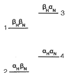
FIG. 2. Energy levels and eigenfunctions of a ^1\text{H} - ^{15}\text{N} spin system.
