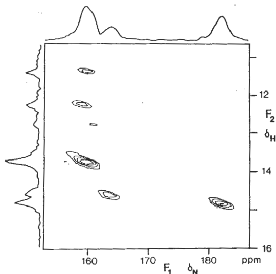
FIG. 10. ^1\text{H} - ^{15}\text{N} shift correlation spectrum of a 0.7 mM 92% \text{H}_2\text{O} /8% \text{D}_2\text{O} solution of \text{tRNA}_{\text{Met}}^{\text{Met}} , labeled with 65% ^{15}\text{N} at N3 of all the uridine related bases in a 200 \mu\text{l} microcell at 15°C. The spectrum was obtained with the sequence of Fig. 1b, and selection of the double quantum component. Due to proton exchange and partial decomposition of the sample, peaks vary in intensity. The peak of the U27-A43 base pair ( \delta_{\text{H}} = 12.7 ppm) disappears at temperatures higher than 15°C. Along the F_1 and F_2 axes, the absolute value mode projections of the 2D spectrum are shown. The total measuring time was 6 hr.
