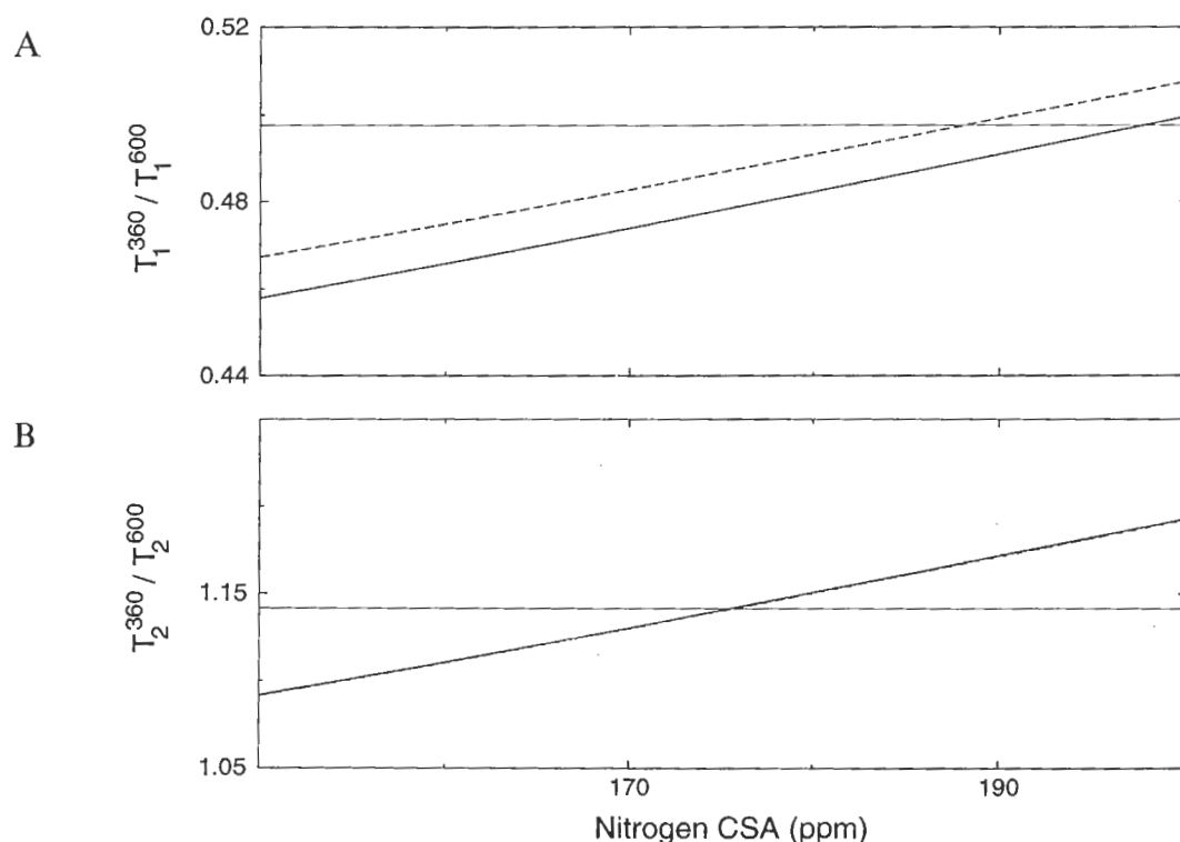
Fig. 6. Theoretical ratio of (A) T_1 values and (B) T_2 values measured at 600 and 360 MHz as a function of the magnitude of the ^{15}\text{N} CSA in the absence of internal motion (solid lines) and in the presence of a 0.04\text{ s}^{-1} 1/T_1 contribution (dashed line) from rapid internal motion. Note that the rapid internal motion does not significantly affect the T_2 ratio, and the dashed line nearly coincides with the solid one in (B). Thin horizontal lines correspond to the experimentally observed average ratios for residues with \text{NOE} > 0.65 , and are not subject to slow conformational exchange.
