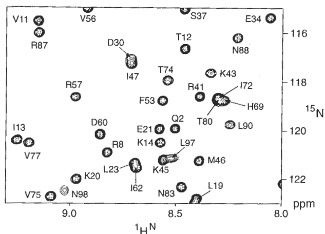
Fig. 1. Small region of the 360 MHz ^1\text{H} - ^{15}\text{N} correlation spectrum of perdeuterated HIV-1 protease, complexed with DMP323, dissolved in 95% \text{H}_2\text{O} /5% \text{D}_2\text{O} . The spectrum corresponds to the first time point of a set of eight such spectra, recorded for measuring the ^{15}\text{N} T_1 .
