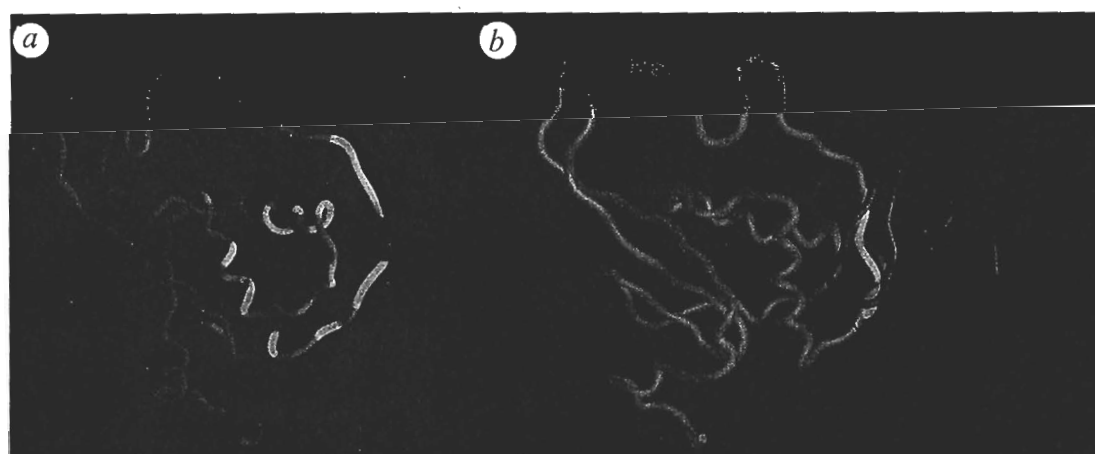
Fig. 3 Model for the interaction of Nef \Delta 2-39, \Delta 159-173 with the SH3 domain of Hck. a , A backbone worm of Nef \Delta 2-39, \Delta 159-173 (residues 56–206) is displayed colour coded to show those residues whose backbone NH, ^{15}\text{N} , ^{13}\text{C}\alpha and ^{13}\text{C}\beta resonances are most affected on binding the SH3 domain of Hck. The mean shift difference \Delta_{\text{ave}} for each amino acid was calculated as 0.25[(\Delta_{\text{NH}})^2 + (\Delta_{\text{N}}/5)^2 + (\Delta_{\text{C}\alpha}/2)^2 + (\Delta_{\text{C}\beta}/2)^2]^{1/2} where \Delta_i is the chemical shift difference for resonance i in the free and complexed states. The colours range from red ( \Delta_{\text{ave}}=1.0 ), through yellow ( \Delta_{\text{ave}}=0.4 ), to blue ( \Delta_{\text{ave}}=0.1 ). Two residues of Nef, Pro 77 and Ala 83, could not be assigned in the complex and are colour-coded in orange. b , A model of the complex obtained by docking the SEM-5-peptide complex 22 onto Nef \Delta 2-39, \Delta 159-173 by best fitting residues 1–7 of the peptide with residues 71–77 of Nef \Delta 2-39, \Delta 159-173 (see text). The colour coding is as follows: Nef \Delta 2-39, \Delta 159-173 , blue; the SH3 domain of SEM-5, red; and the nine-residue peptide (PPPVPVRRR) from mSos, yellow. This figure was generated with the program GRASP 33 .
