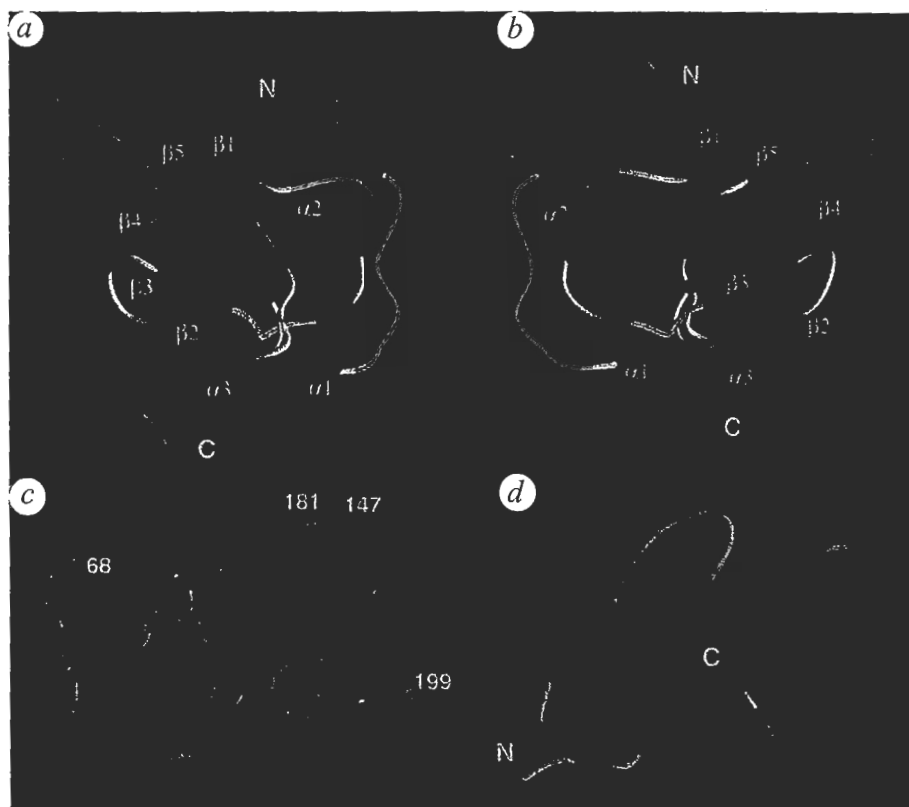
Fig. 2 a and b , Two views showing a backbone ribbon diagram of Nef \Delta 2-39, \Delta 159-173 (residues 56–206). c , Packing of the hydrophobic core of Nef \Delta 2-39, \Delta 159-173 . d , Backbone ribbon diagram of GH5 21 in the same orientation as ( b ) showing the similar fold to Nef \Delta 2-39, \Delta 159-173 . The colour coding in ( a ), ( b ) and ( d ) is as follows: helices, red; \beta -strands, green; polyproline helix and helical turn preceding strand \beta 2 , yellow; ordered loops, grey; and disordered regions, blue. In ( c ) the backbone for residues 68–147 and 181–199 is shown as a green worm and the internal side chains are shown in red. ( a ), ( b ) and ( d ) were generated with the program RIBBONS 32 and ( c ) with the program GRASP 33 .
