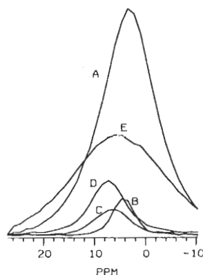
FIG. 3. Proton frequency cross sections for five different carbon chemical shifts. Cross sections A through E correspond to ^{13}\text{C} chemical shifts of 16.1, 64.4, 112.9, 117.8, and 154.2 ppm, respectively.
