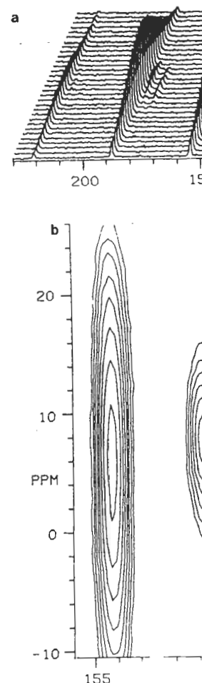
FIG. 2. The results of the refocussing experiment. For details of the conditions, see under Experimental. The cross section of Fig. 2a is shown for the center of the spectrum.
