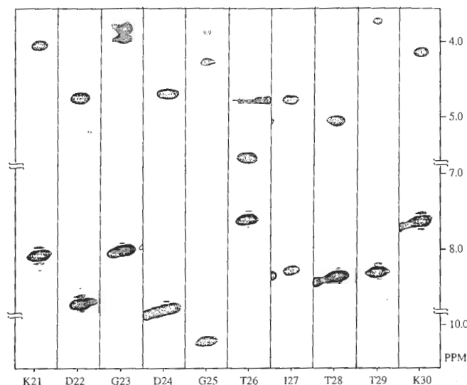
Fig. 4. F_1 strips taken from the 3D HNHA spectrum of calcium-free calmodulin for residues Lys 21 -Lys 30 . The 3D spectrum results from a 70^* \times 47^* \times 512^* data matrix, with acquisition times of 15.4 ( t_1 ), 38 ( t_2 ) and 55 ( t_3 ) ms. Acquired data were apodized with a 65^\circ -shifted squared sine-bell in the t_3 dimension, truncated at 10% ( \sin^2 162^\circ ) at the end of the FID, and with a 68^\circ -shifted sine-bell in the t_1 dimension, also truncated at 10% (at \sin 174^\circ ). Truncation at the end of the sine-bell is used as a compromise between maximizing spectral resolution (and sensitivity) and minimizing truncation artifacts. The t_2 ( ^{15}\text{N} ) time domain data has been extended to 83^* data points by mirror-image linear prediction, prior to apodization with a squared cosine-bell and zero-filling to 128^* . Digital resolutions in the final 3D spectrum were 17.7 ( F_1 ), 9.6 ( F_2 ) and 4.5 ( F_3 ) Hz. Total acquisition time was 32 h.
