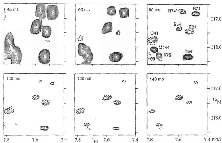
Fig. 2. Small sections of the CT-HMQC-J spectra of \text{Ca}^{2+} -free calmodulin, recorded with the pulse scheme of Fig. 1A, using dephasing periods ( 4T + 2\Delta ) of 45, 60, 80, 100, 120 and 140 ms. Each spectrum results from 64 scans per complex t_1 increment and the total recording time for the six spectra was 12 h. The acquired data matrices contain 38, 56, 81, 106, 131 and 156 complex data points in the t_1 dimension. For all six spectra mirror-image linear prediction (using 16 coefficients) was used to double the duration of the t_1 time domain (Zhu and Bax, 1990), prior to apodization with a squared cosine-bell window function. All spectra were zero-filled to yield digital resolutions of 2.4 ( F_1 ) and 9.0 ( F_2 ) Hz.
