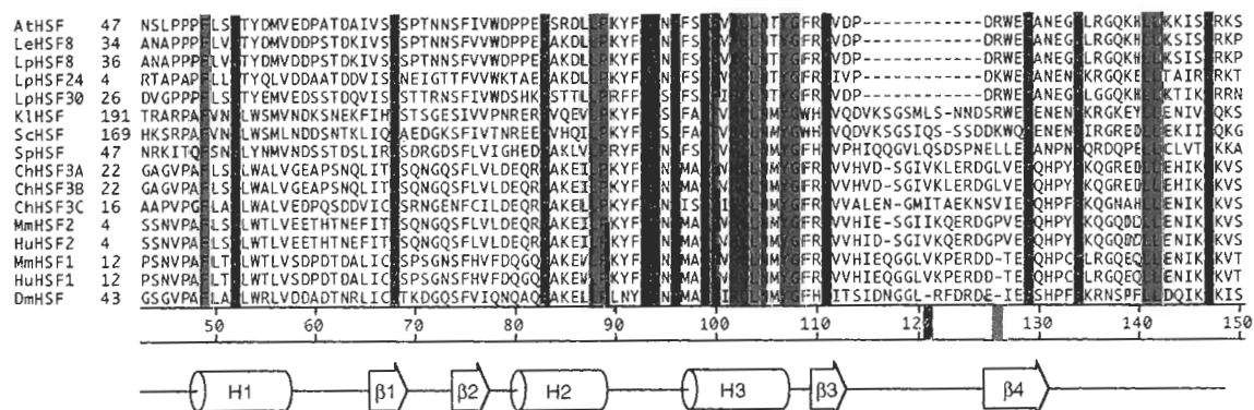
Fig. 1 Alignment of HSF DNA-binding domain sequences from Arabidopsis thaliana (AtHSF) 31 , Lycopersicon esculentum (LeHSF) 34 , Lycopersicon peruvianum (LpHSF 8 , 24, and 30) 32 , Kluyveromyces lactis (KlHSF) 33 , Saccharomyces cerevisiae (ScHSF) 34 , Schizosaccharomyces pombe (SpHSF) 35 , Gallus gallus (ChHSF) 36 , Mus musculus (MmHSF1 and 2) 37 and Human (HuHSF1 and 2) 38,39 to the Drosophila melanogaster (DmHSF) 22 DNA-binding domain using the CLUSTAL-V algorithm 40 . Absolutely conserved polar and ionic residues are highlighted in red, while absolutely conserved hydrophobic residues are highlighted in green. Secondary structural elements for dHSF residues 43–148 are shown below the sequence alignment.
