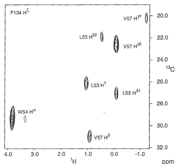
Fig. 2 Small region of a F 1 /F 2 cross section, at the F 3 frequency of Phe 134 H ε , through the 3D 13 C-edited, 12 C-filtered HMQC-NOESY experiment. The 3D spectrum was recorded in 38 h for a 2 mM solution of [ 12 C-Phe, U- 13 C/ 15 N] reverse-labelled dHSF(33–155) in D 2 O (ref. 9). 1 H– 13 C correlations are seen for all protons that experience an NOE interaction with Phe 134 H ε . The spectral window in the 13 C dimension is 33.1 p.p.m. and the Trp 54 H α resonance is folded once.
