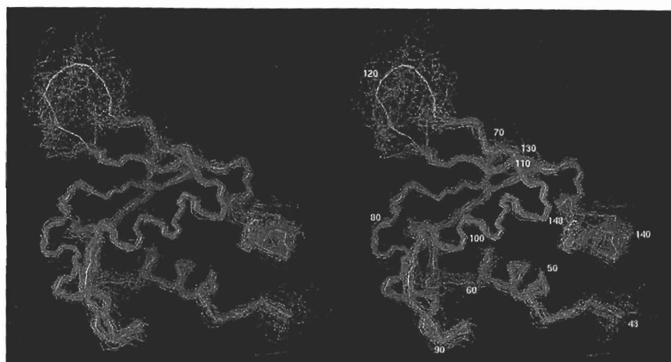
Fig. 3 Best-fit superposition of the backbones of the 28 simulated annealing structures (blue) and the refined average structure of dHSF-DBD (yellow).
