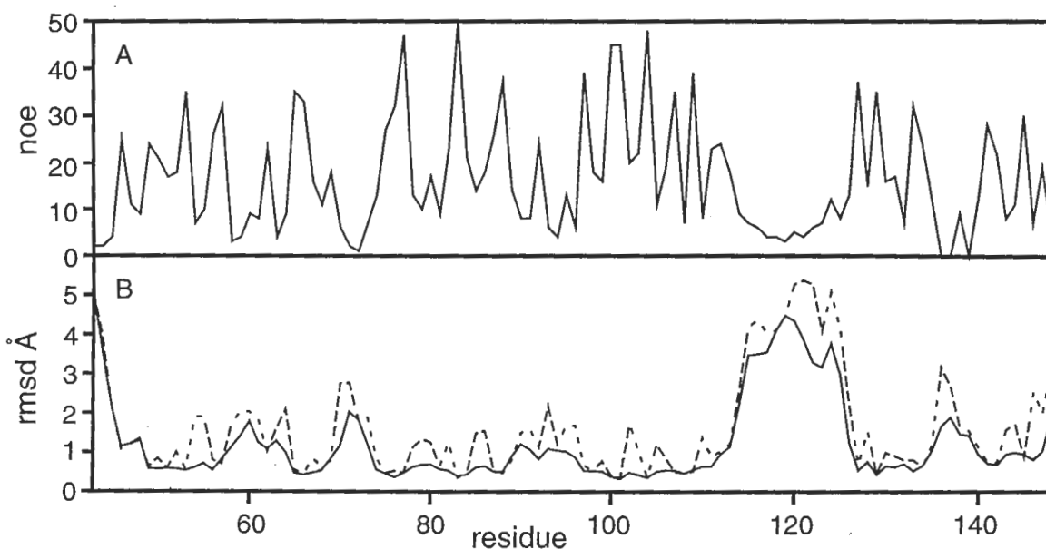
Fig. 4 a, Total number of sequential, medium-range, and long-range restraints per residue and b, positional r.m.s.d. values per residue for the backbone (solid lines) and all heavy atoms (dashed lines). Restraints are counted for both donor and acceptor atoms. R.m.s.d. values are calculated from the 28 refined structures.
