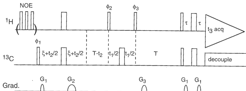
Fig. 3. Pulse scheme of the 3D LRCH experiment. Narrow rectangles correspond to pulses with a 90^\circ flip angle, wide rectangles to 180^\circ . Unless indicated otherwise, pulses are applied along the x axis. During the 700 ms delay between scans, 120^\circ proton pulses, separated by 10 ms intervals, are used for obtaining NOE enhancement of the ^{13}\text{C}^\epsilon methyl magnetization. Delay durations: \xi = 0.9 ms, \tau = 1.75 ms; T = 19.6 ms. G_{1,2,3} = 0.3, 0.8 and 0.5 ms. Phase cycling: \phi_1 = y, -y ; \phi_2 = x, x, -x, -x ; \phi_3 = 4(x), 4(-x) ; Receiver = x, -x, -x, x, -x, x, x, -x . For the 2D reference spectrum, t_1 is kept at 2\ \mu\text{s} , and Receiver = x, -x , with phase cycling for \phi_1, \phi_2 and \phi_3 the same as for the 3D experiment. Quadrature in the t_1 and t_2 dimensions is obtained by incrementing \phi_2 and \phi_1 in the regular States-TPPI manner.
