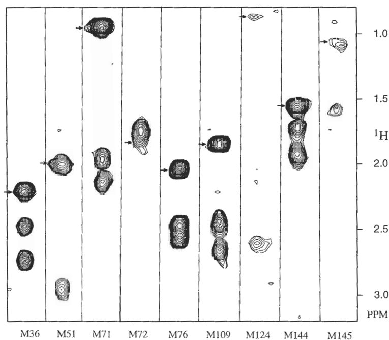
Fig. 7. F_1 strip plot of the 3D LRCH spectrum of the calmodulin-M13 complex, showing the correlation between \text{C}^\epsilon/\text{H}^\epsilon and \text{H}^\gamma resonances for the methionine residues. Spurious diagonal resonances ( F_1 = F_3 = \delta\text{H}^\epsilon ) are marked by arrows. Contours are spaced exponentially by 2^{1/3} .
