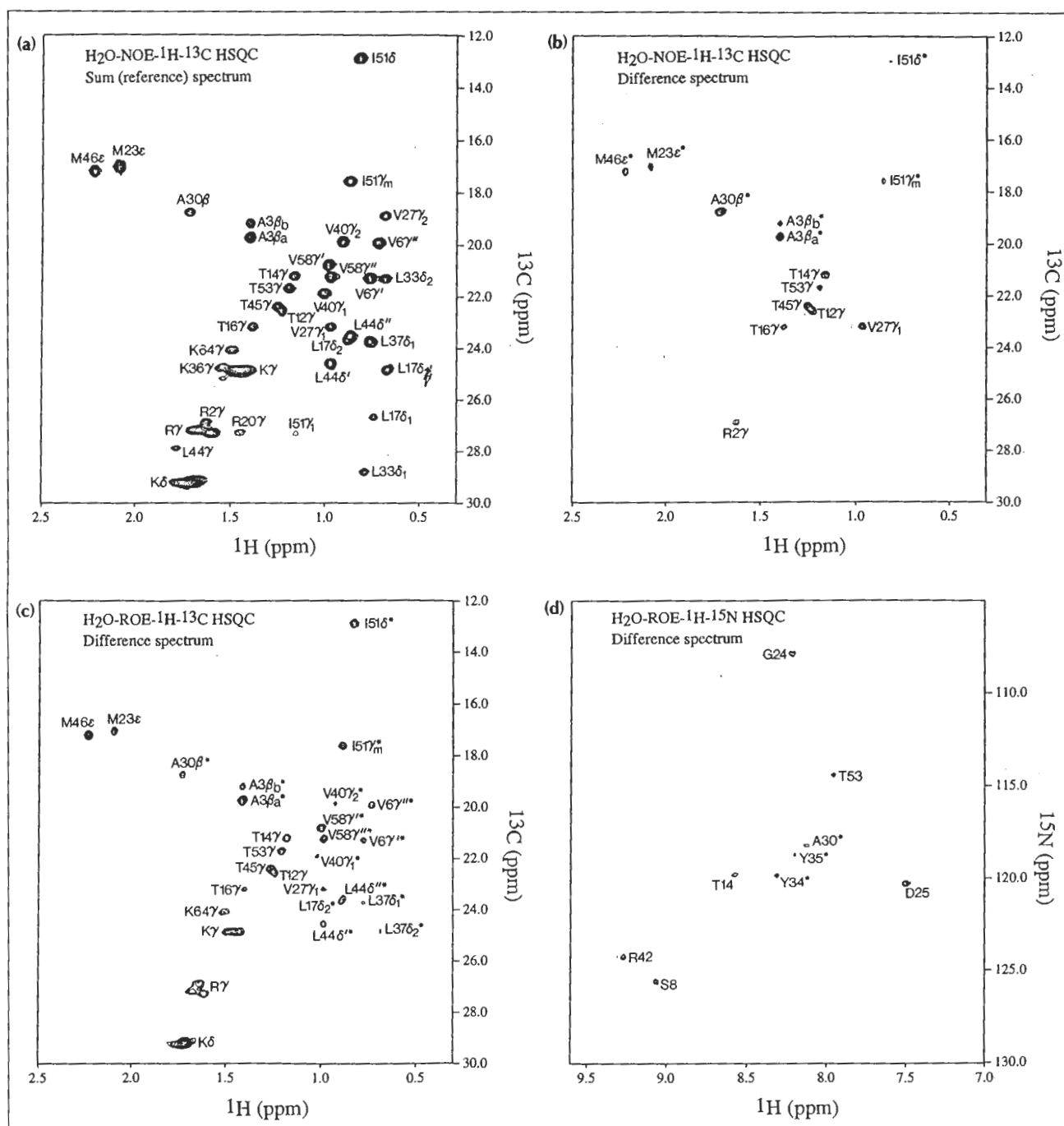
Fig. 1. Portions of the NOE and ROE spectra of the specific chicken GATA-1-DNA complex recorded with NOE/ROE mixing times of 60 ms at 25 °C. (a) The reference (i.e. sum) H 2 O-NOE- ^1\text{H} - ^{13}\text{C} HSQC spectrum. (b) The difference H 2 O-NOE- ^1\text{H} - ^{13}\text{C} HSQC spectrum. (c) The difference H 2 O-ROE- ^1\text{H} - ^{13}\text{C} HSQC spectrum. (d) The difference H 2 O-ROE- ^1\text{H} - ^{15}\text{N} HSQC spectrum. Positive and negative contours are shown as continuous and dashed lines, respectively. Cross-peaks that can be attributed unambiguously to an NOE/ROE to bound water are indicated by an asterisk in panels (b) to (d); for all other peaks an indirect mechanism involving an NOE/ROE to a rapidly exchangeable proton followed by chemical exchange with water cannot be excluded. In (a), peaks involving a carbon atom attached to an even or odd number of neighboring carbon atoms are of opposite sign and are displayed as negative and positive contours, respectively. The sign of the ROE is always positive and opposite to that of the peaks observed in the reference spectrum (which are equivalent to the diagonal in a regular homonuclear 2D ^1\text{H} - ^1\text{H} NOE spectrum). The sign of the NOE depends on the residency time of the water. With the exception of the methyl group of Met23, all the NOEs peaks are of the same sign as the peaks in the reference spectrum, i.e. the sign is negative, and hence the residency times of the bound water molecules are greater than 300 ps. In (d), only positive contours corresponding to ROEs are displayed; the spectrum also contains negative contours which arise from chemical exchange between rapidly exchanging amide groups and water. In panels (a), (b) and (c), note that there are two resonances for the methyl protons of Ala3 due to amino-terminal heterogeneity; in addition, methyl groups of valine and leucine that are not stereo-assigned (due to the presence of multiple rotamer conformations) are denoted by the superscripts prime and double prime. The reference (sum) spectrum in (a) is plotted at a 37.5 times higher contour level than the corresponding difference spectrum in (b).
