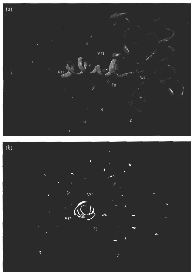
Fig. 4. (a,b) Two orthogonal views of a schematic ribbon drawing representation of the solution NMR structure of the \text{Ca}^{2+} -CaM-M13 complex, with the amino-terminal domain in blue, the carboxy-terminal domain in purple, and the M13 peptide in yellow. The hydrophobic side chains of the amino- and carboxy-terminal domains of CaM are shown in red, and the Trp4, Phe8, Val11 and Phe17 side chains of the peptide are displayed in green. The model was generated using the program VISP (written by E de Castro and S Edelstein), and the coordinates were taken from [16 • ].
