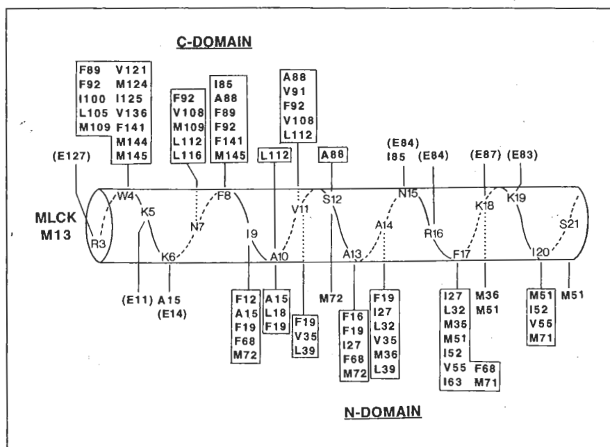
Fig. 5. Summary of residue pairs for which intermolecular NOEs between CaM and M13 are observed. CaM residues involved in hydrophobic interactions are boxed. Also included are potential electrostatic interactions between negatively charged glutamate residues of CaM, shown in parentheses, and positively charged lysine and arginine residues of M13; it should be noted that the electrostatic interactions have been inferred purely from the structure as no NOEs have been identified between these pairs of residues. Adapted from [16**].
