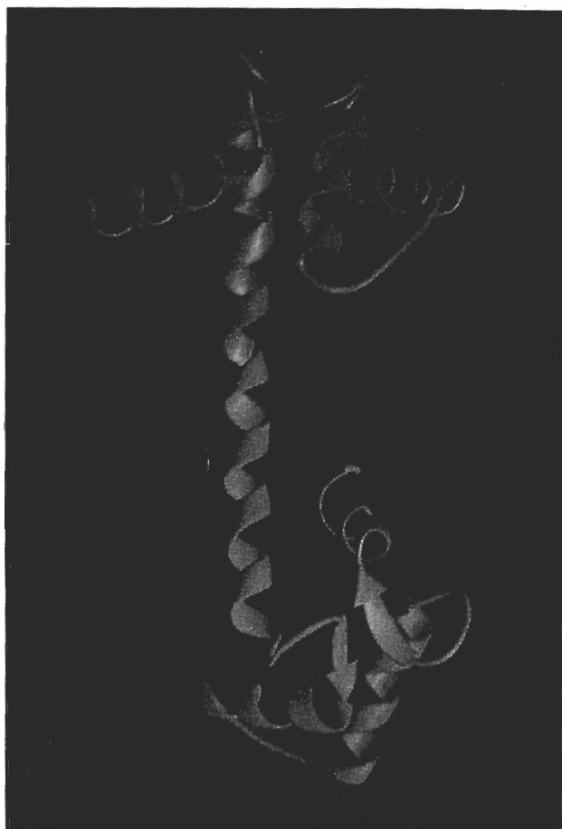
Fig. 1. Ribbon drawing of the X-ray structure of uncomplexed \text{Ca}^{2+} -CaM [6]. The amino terminal domain is shown in blue and the carboxy terminal one in red. The model was generated with the program RIBBONS (written by M Carson).
