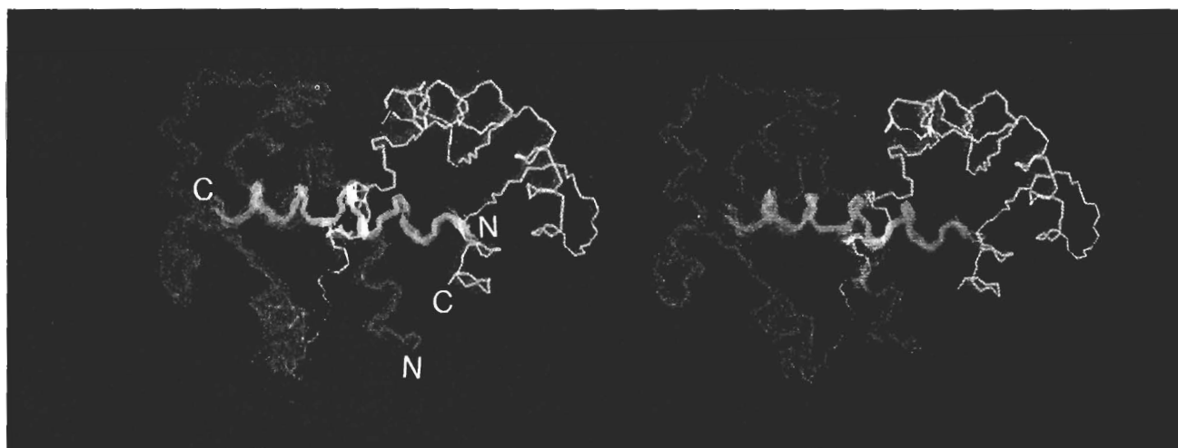
Fig. 2. Stereoview showing a best-fit superposition of the backbone (N, \text{C}_\alpha , C) atoms of an ensemble of 24 calculated structures of the \text{Ca}^{2+} -CaM-M13 complex determined by NMR spectroscopy. The amino-terminal domain is shown in blue, the carboxy-terminal domain in red, and the M13 peptide in green; the restrained regularized mean structure is also included in the superposition and is highlighted. The coordinates were derived from [16*].
