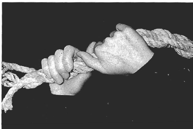
Fig. 3. Schematic representation of the structure of the \text{Ca}^{2+} -CaM-peptide complex, in which the peptide is represented by a rope, and the two domains of CaM by two right hands.
