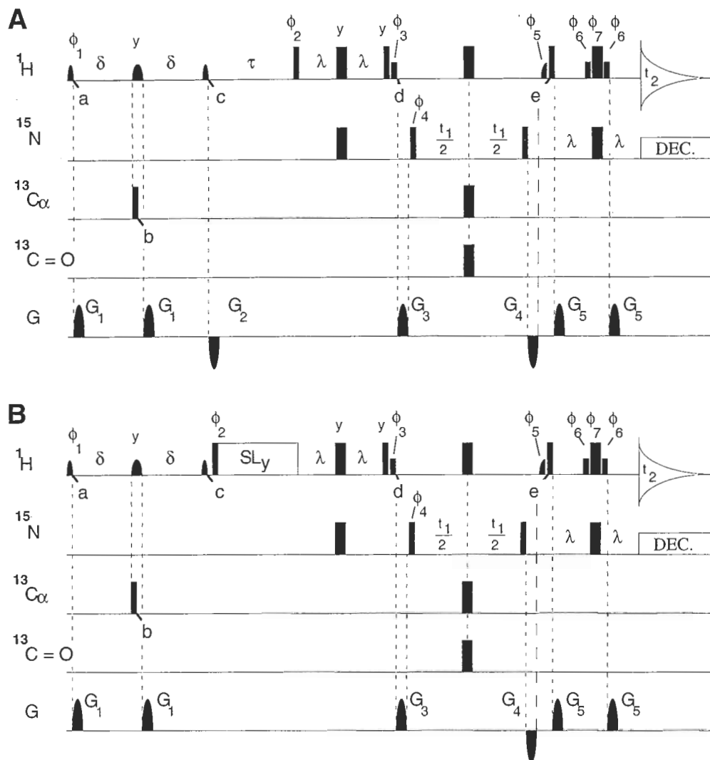
Fig. 1. Pulse scheme of the water-NOE (A) and water-ROE (B) experiments. Narrow and wide pulses correspond to 90^\circ and 180^\circ flip angles, respectively. Pulses for which the phase is not indicated are applied along the x-axis. The ^1\text{H} carrier frequency is set to the \text{H}_2\text{O} frequency, the ^{15}\text{N} , ^{13}\text{C}\alpha and ^{13}\text{C}=\text{O} carrier frequencies are set to 116.5, 56 and 177 ppm, respectively. ^{15}\text{N} decoupling is accomplished using WALTZ-16 modulation with a 1.5 kHz RF field. The first three ( 90^\circ , 180^\circ , 90^\circ ) ^1\text{H} pulses each have the shape of the center lobe of a (\sin x)/x function and a duration of 2 ms for the 90^\circ pulses. The 90^\circ_{\text{ss}} ^1\text{H} pulse has the profile of the left half of a Gaussian function and a width at half height of 500 \mu\text{s} . All other ^1\text{H} pulses are rectangular in shape. Their RF field strength is 270 Hz for the 90^\circ_{\text{ss}} and 90^\circ_{\text{ss}} pulses and 27 kHz for all other ^1\text{H} pulses. The 90^\circ ^{13}\text{C}\alpha pulse is applied at high power ( \gamma B_1/2\pi = 15 kHz); the 180^\circ ^{13}\text{C}\alpha and ^{13}\text{C}=\text{O} decoupling pulses are applied at reduced power ( \gamma B_1/2\pi = 4.7 kHz). Pulsed field gradients have a sine-bell amplitude profile with a strength of 25 G/cm at their center. Their durations are G_{1,2,3,4,5} = 0.5, 10.0, 2.5, 1.0, 0.4 ms. Delay durations are \delta = 2.4 ms, \tau = 60 ms, \lambda = 2.25 ms. Phase cycling of scheme (A) is as follows: \phi_1 = x ; \phi_2 = 4(x), 4(-x) ; \phi_3 = 4(-x), 4(x) ; \phi_4 = x, -x ; \phi_5 = -x ; \phi_6 = 2(-x), 2(x) ; \phi_7 = 2(x), 2(-x) . Acq. = 2(x, -x), 2(-x, x) . Quadrature in the t_1 domain is obtained by changing the phase \phi_4 in the usual States-TPPI manner (Marion et al., 1989). For the difference experiment, two sets of data are recorded in an interleaved manner with phases \phi_1 and \phi_3 either set to the values above, or inverted by 180^\circ . For scheme (B) all parameters are the same as for (A). The additional spin-lock pulse along the y-axis, \text{SL}_y , has an RF field strength of 10 kHz and a duration of 25 ms.
