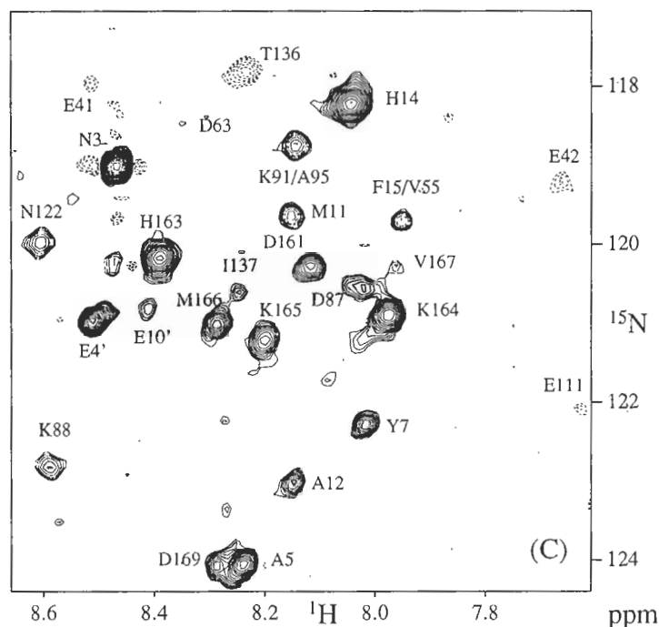
Fig. 2. Small regions of the water-protein NOE and ROE HSQC difference spectra recorded with the pulse schemes of Fig. 1 for the protein calceinurin B. (A) NOESY difference spectrum, recorded with a 60-ms mixing time (total acquisition time 14.5 h). (B,C) ROESY difference spectra, recorded with 25-ms (B) and 100-ms (C) mixing time (total acquisition times of (B) 14.5 h and (C) 6.5 h). Dashed contours indicate negative resonances. Contours are spaced by a factor of 1.25.
