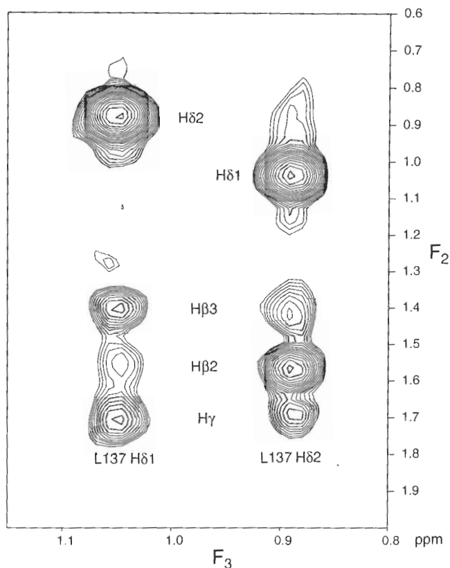
Fig. 2. Two F_2 strips from the 3D ^1\text{H} -detected [ ^{13}\text{C} - ^1\text{H} ] long-range correlation of SNase, recorded with the pulse sequence of Fig. 1, using 2T = 31.6 ms, centered at the ^{13}\text{C} ( F_1 ) and ^1\text{H} ( F_3 ) frequencies of the \delta_1 and \delta_2 methyl groups of Leu 137 . The strips display correlations to all protons with a significant J coupling to \text{C}_{\delta_1} (left strip) and \text{C}_{\delta_2} (right strip).
