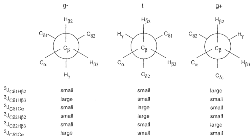
Fig. 3. Newman projections illustrating the \chi_2 torsion angle in leucine. The \chi_2 torsion angle and prochiral H_\beta and C_\delta H_3 have been defined in accordance with IUPAC rules (IUPAC-IUB Commission on Biochemical Nomenclature 1970).
