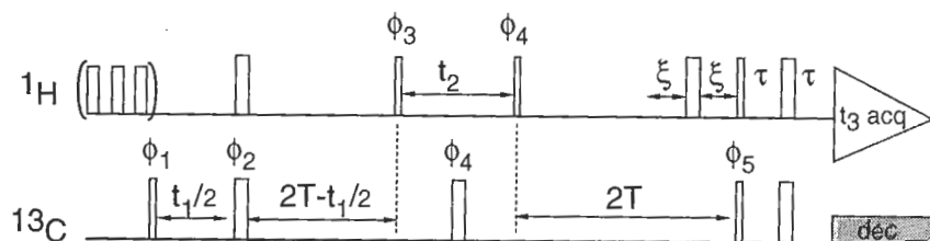
Fig. 1. Pulse sequence of the 3D ^1\text{H} -detected [ ^{13}\text{C} - ^1\text{H} ] long-range correlation experiment. Narrow and wide pulses denote 90^\circ and 180^\circ flip angles, respectively. The pulse train on the ^1\text{H} channel during the relaxation delay consists of low-power 135^\circ pulses spaced by 10-ms delays and serves to build up the heteronuclear NOE. The carrier for the carbon 90^\circ and 180^\circ pulses was positioned at 25 ppm. Unless indicated otherwise, all pulses are applied along the x-axis. The phase cycle is as follows: \phi_1 = x ; \phi_2 = 4(x), 4(y), 4(-x), 4(-y) ; \phi_3 = x, -x ; \phi_4 = 2(x), 2(-x) ; \phi_5 = 16(y), 16(-y) , receiver = P, -P, P, -P, -P, P, -P, P, with P = (x, -x, -x, x). The 2D reference spectrum was recorded by setting t_2 = 0 , and using the following receiver phase cycle: 4(x), 4(-x), 4(x), 8(-x), 4(x), 4(-x), 4(x) . Quadrature detection in t_1 and t_2 is obtained by the States-TPPI method (Marion et al., 1989) by incrementing phases \phi_1 and \phi_3 , respectively. Delay durations: \tau = 1.7 ms, 2T = 15.8, 23.7 , or 31.6 ms, and \xi = 1 ms.
