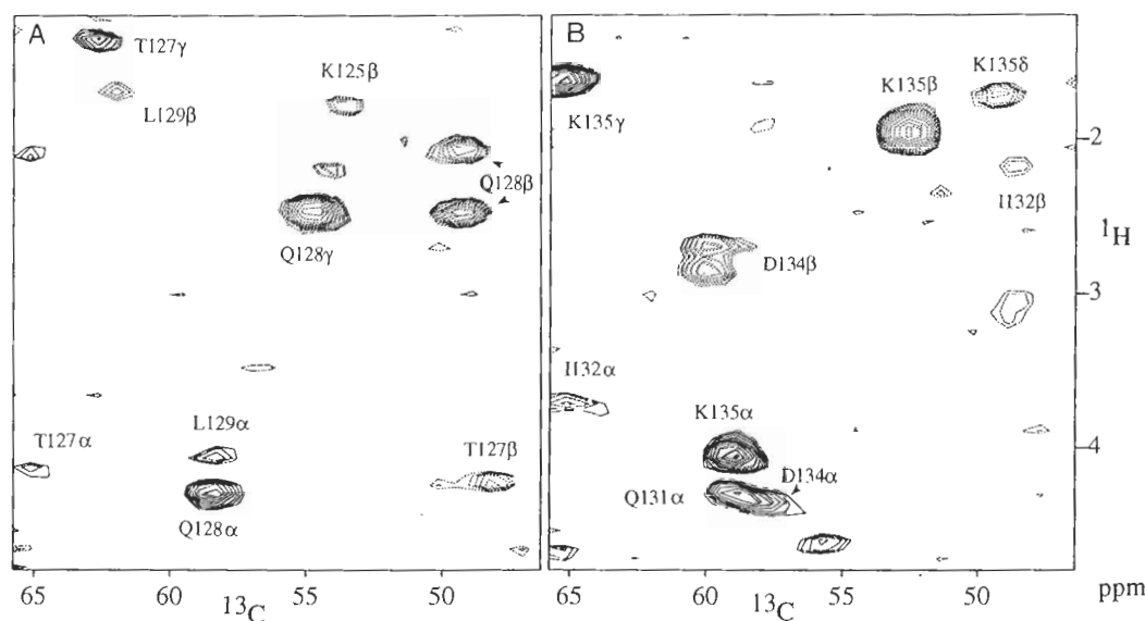
Fig. 3. Two 'strips' taken from the 600-MHz 4D ^{15}\text{N}/^{13}\text{C} -separated NOESY spectrum of calcineurin B, 2.3 mM in the presence of 25 mM CHAPS, dissolved in 5% \text{D}_2\text{O}/95\% \text{H}_2\text{O} , pH 4.9, displaying the interaction between aliphatic resonances and (A) the amide of Gln 128 and (B) the amide of Lys 135 . Dashed contours correspond to resonances with negative intensity, caused by aliasing an odd number of times in the ^{13}\text{C} dimension.
