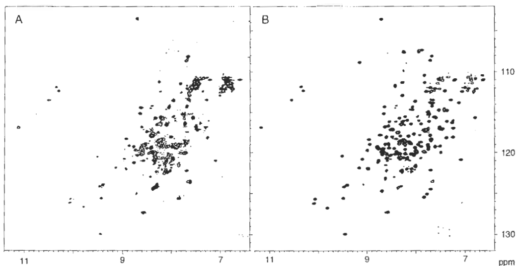
Fig. 2. ^1H - ^{15}N correlation spectra of 5% D_2O /95% H_2O solution of 0.8 mM ^{15}N -labeled calcineurin B at 35 °C, pH 4.9, in (A) the absence and (B) the presence of 18 mM CHAPS. Spectra were recorded at 600-MHz ^1H frequency, on a Bruker AMX-600 spectrometer. Acquisition times in the t_1 (102.8 ms) and t_2 (120.8 ms) dimensions and the total number of scans and measuring time (2 h per spectrum) were identical for both spectra. Both data sets were processed with identical digital filtering (squared sine shifted by 45° in the t_1 dimension and by 60° in the t_2 dimension), and both data sets were zero filled to yield a 512 x 1024 matrix size for the absorptive part of the 2D spectrum.
