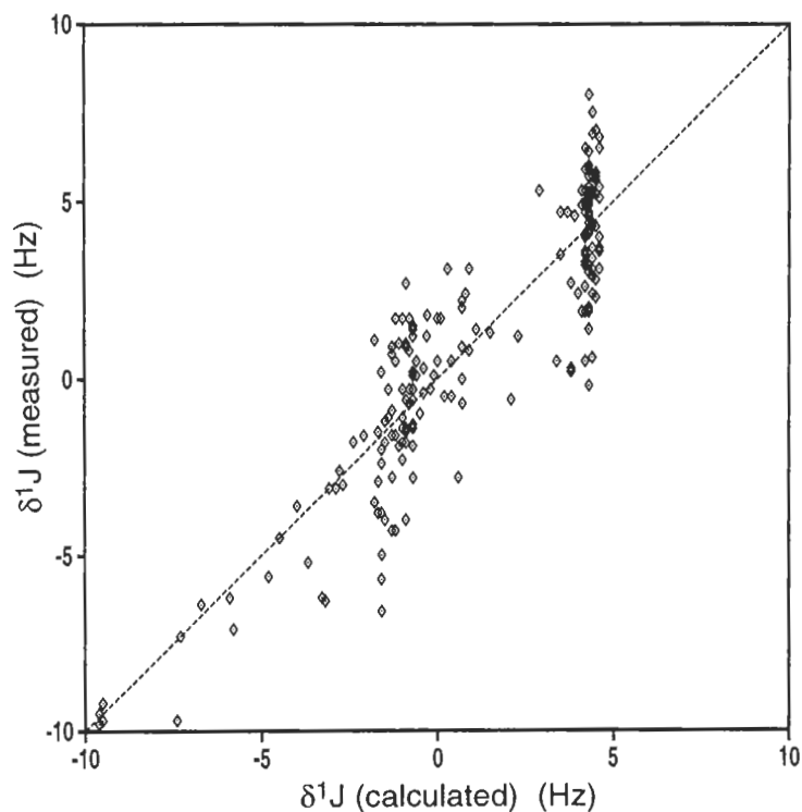
Fig. 4. Measured \delta^1J versus \delta^1J expected on the basis of the \Delta^1J(\phi, \psi) distribution of Fig. 2. The r.m.s.d. is 1.6 Hz.
