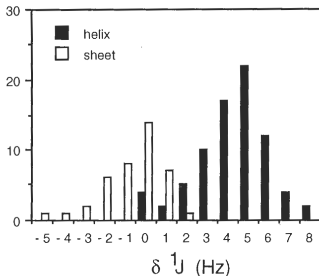
Fig. 3. Histogram of the \delta^1J values for residues in \alpha -helical and \beta -sheet conformation.
