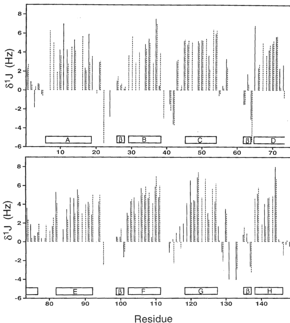
Fig. 5. Measured \delta^1J values for CaM (solid lines) and the CaM/M13 complex (broken lines). Indicated are the secondary structural elements for CaM as inferred from previous NMR studies (Ikura et al., 1991b); A–H denote \alpha -helices, \beta denotes anti-parallel \beta -sheet.
