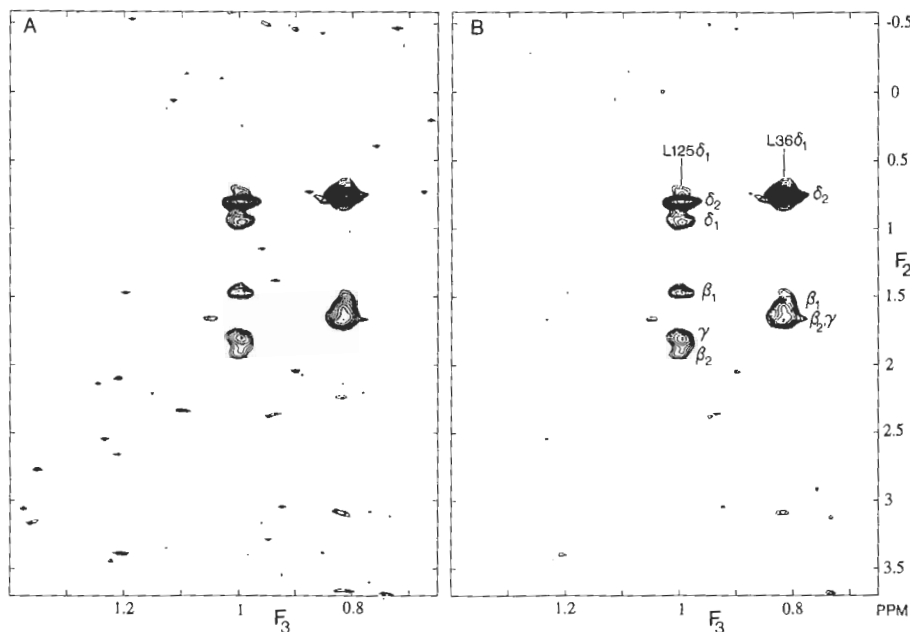
FIG. 2. Comparison of spectra obtained by extending the t_2 time domain eightfold using (A) regular LP and (B) FB-LP. In both cases, 10 coefficients were used and data were extended from 32 complex to 256 complex. Data shown correspond to an F_2/F_3 slice through a 3D spectrum of S. nuclease, enriched with ^{13}\text{C} in the \text{C}_\delta position of Leu residues, showing correlations between methyl protons and other protons that have a significant ( \geq 2 Hz) J coupling to the methyl ^{13}\text{C} .
