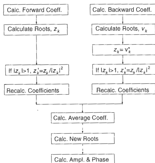
FIG. 1. Flow diagram of the forward-backward linear prediction procedure. The left part of the scheme is used in regular linear prediction; v_k^* is the complex conjugate of v_k . The last two steps, recalculation of the new roots from the averaged coefficients and determination of the amplitude and phase of the frequency components, are omitted when the method is used simply to extend the length of the FID.
