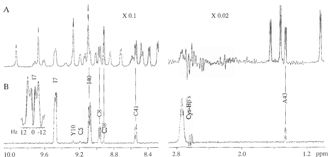
Fig. 2. Selected regions of the ^1\text{H} NMR spectrum of ^{199}\text{Hg} -substituted rubredoxin, acquired with the spin-echo sequence described in the text. Except for the differences mentioned in the text, the spectra were recorded under the same conditions as in Fig. 1. The downfield and upfield regions of the ^1\text{H} spectrum shown in (A) are displayed at 0.1- and 0.02-fold magnification compared to (B), after correction for the number of transients. Inset: ^1\text{H} - ^{199}\text{Hg} J splitting for 17-H _N resolved by strong resolution enhancement.
