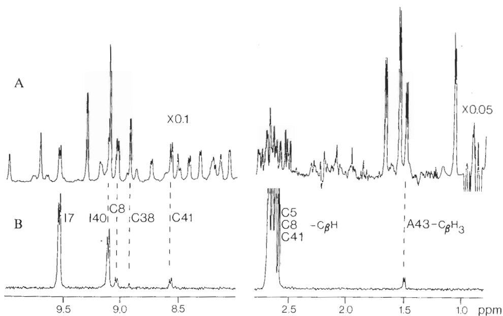
Fig. 1. Selected regions of the ^1\text{H} NMR spectrum of ^{113}\text{Cd} -substituted rubredoxin, acquired with the spin-echo sequence described in the text. (A) Spectrum obtained using the first 4 steps of the phase cycle, i.e., without affecting the ^{113}\text{Cd} spin state. The spectrum results from 1200 transients. (B) Spectrum obtained using the full 8-step phase cycle spin-echo difference experiment with identical parameters compared to (A) except for the number of transients (120 000 total, 60 000 with \phi_2 = x , and 60 000 with \phi_2 = -x ). The total measuring time was \sim 36 h. The downfield and upfield regions of the ^1\text{H} spectrum shown in (A) are displayed at 5- and 2.5-fold higher magnification compared to (B), 0.1- and 0.05-fold after correction for the number of transients.
