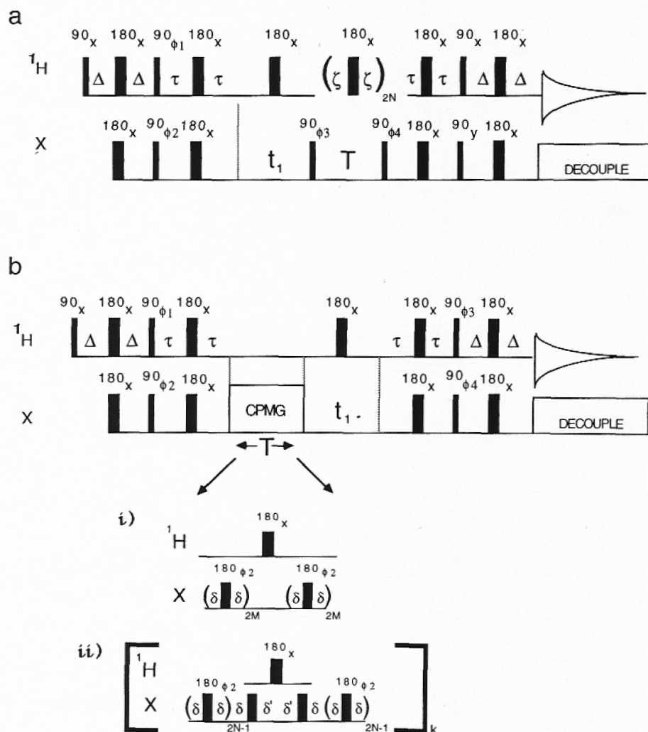
FIG. 2. Pulse sequences for measuring heteroatom T_1 (a) and T_2 relaxation times (b). Effective water suppression (if X = {}^{15}\text{N} ) is achieved with the use of an off-resonance DANTE sequence (31, 32). The value of \Delta is set to slightly less than 1/(4J) , where J is the {}^1\text{H} - X coupling constant (2.3 ms for X = {}^{15}\text{N} ) to minimize relaxation losses. Because the transverse relaxation times for backbone {}^{15}\text{N} spins are reasonably long, the value of \tau is set to 1/(4J) . In a, {}^1\text{H} 180^\circ pulses are applied every 5–10 ms (at a rate much greater than the decay rate of the fastest relaxing multiplet component) in order to suppress the effects of {}^1\text{H} - {}^{15}\text{N} dipolar/CSA cross correlation. The phase cycling employed is \phi_1 = 8(y), 8(-y) ; \phi_2 = 4(x), 4(-x) ; \phi_3 = -y, y ; \phi_4 = 2(x), 2(-x) ; Acq = x, 2(-x), x, -x, 2(x), -x . The receiver phase is inverted every eight scans. A composite 180^\circ pulse ( 90_x 180_y 90_x ) is applied in the center of the t_1 evolution period. Quadrature in F_1 is achieved by TPPI (33) of \phi_3 . In b, the pulse scheme for measuring heteroatom T_2 values published previously (i) and the new sequence which completely suppresses the effects of {}^1\text{H} - {}^{15}\text{N} dipolar/ {}^{15}\text{N} CSA cross correlation (ii) are indicated. The modified CPMG sequence (ii) consists of applying {}^1\text{H} 180^\circ pulses every 5–10 ms at the peak of the spin echo in order to invert the {}^1\text{H} spin state and hence average the relaxation rates of the multiplet components. Note that {}^1\text{H} 180^\circ pulses are positioned such that {}^{15}\text{N} magnetization spends an equal amount of time associated with each of the multiplet components. The delay \delta' is chosen such that 2\delta' + \delta_{\text{H}180^\circ} = 2\delta ( \delta_{\text{H}180^\circ} = {}^1\text{H} 180^\circ pulse width) with the value of \delta set < 1/(2J) so that
