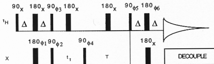
FIG. 3. Scheme for the measurement of T_{1zz} . For the case in which spectra are recorded in water (i.e., where X = {}^{15}\text{N} ), effective water suppression is achieved with the use of an off-resonance DANTE sequence described previously (32). In addition, a 180^\circ {}^1\text{H} pulse is applied in the center of the relaxation period, T , so that any water magnetization that relaxes along z is inverted. In this way at the end of T very little net water magnetization is along the z axis. The value of \Delta is set to 2.3 ms. The phase cycling employed is \phi_1 = 4(x), 4(-x) ; \phi_2 = x, -x ; \phi_3 = 2(y), 2(-y) ; \phi_4 = 16(x), 16(-x) ; \phi_5 = 8(x), 8(-x) ; \phi_6 = 4(x), 4(y) ; \text{Acq} = x, 2(-x), x, -x, 2(x), 2(-x), 2(x), -x, x, 2(-x), x . The phase of the receiver is inverted every 16 scans. A composite 180^\circ pulse is applied at the center of the t_1 evolution period. Quadrature in F_1 is achieved by TPPI of \phi_2 .
