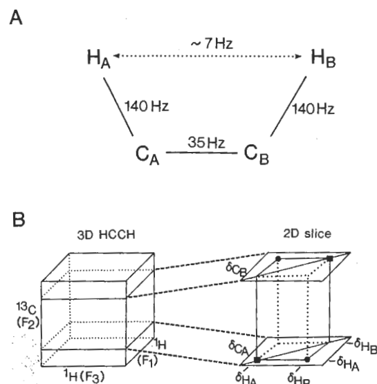
FIGURE 1: (A) Schematic representation of the ^1\text{H} - ^{13}\text{C} - ^1\text{H} spin system with typical coupling constants of ^1J_{\text{CC}} , ^1J_{\text{CH}} , and ^3J_{\text{HH}} . (B) Schematic diagram of a 3D HCCH spectrum and its two slices at the ^{13}\text{C} ( F_2 ) chemical shifts of the nuclei \text{C}_A and \text{C}_B , showing the diagonal and cross peaks expected for the simple spin system. The diagonal peaks are represented by squares and the cross peaks by circles.
