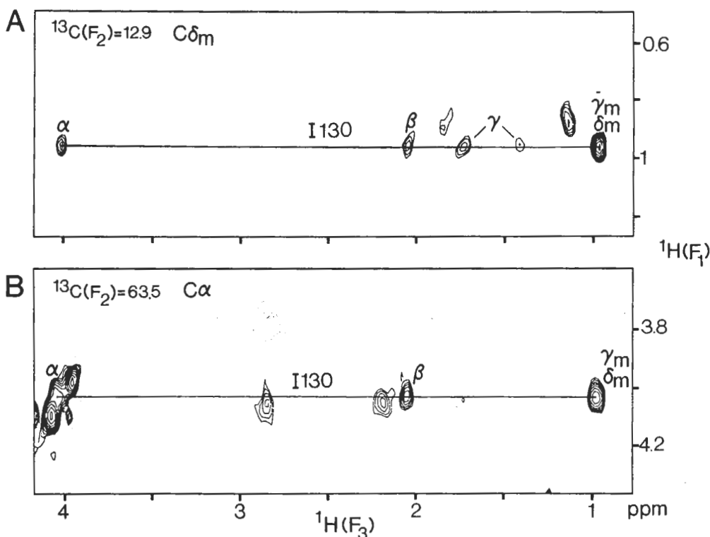
FIGURE 5: Selected slices at different ^{13}\text{C} ( F_2 ) chemical shifts of the 24-ms HCCH-TOCSY spectrum of uniformly ^{15}\text{N} - and ^{13}\text{C} -labeled CaM illustrating the mirror image cross peaks originating from the \text{C}\alpha\text{H} and \text{C}\delta\text{H}_3 protons of Ile-130. A similar connectivity pattern was observed in the slices corresponding to the ^{13}\text{C}\beta (38.7 ppm), ^{13}\text{C}\gamma (28.3 ppm), and ^{13}\text{C}_{\gamma\text{m}} (17.6 ppm) of Ile-130.
