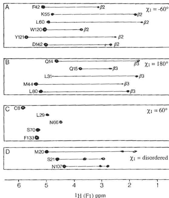
Fig. 4. Composite of amide strips taken from the 3D ^{15}\text{N} -separated HOHAHA-HMQC spectrum of ^{15}\text{N} labeled IL-1 \beta recorded with a 30.7 ms mixing time showing NH-C H and NH-C β H cross peaks for a number of residues. Examples of residues with \chi_1 = -60^\circ , 180^\circ and 60^\circ are shown in (A), (B) and (C), respectively, while residues with disordered \chi_1 conformations are shown in (D). The strips were extracted from the 3D spectrum as described by Driscoll et al. (1990a). The assignments are from Driscoll et al. (1990a) and Clore et al. (1990c).
