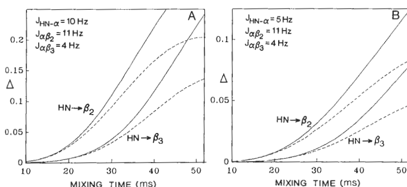
Fig. 1. Fraction of magnetization, \Delta , transferred from the HN to the C^{\beta 2} H and C^{\beta 3} H protons as a function of the duration of isotropic mixing for (A) ^3J_{HN\alpha} = 10 Hz and (B) ^3J_{HN\alpha} = 5 Hz. For both cases ^2J_{\beta 2\beta 3} = -14 Hz. Ideal isotropic mixing is assumed and the fractions are calculated in the absence of relaxation. Relaxation attenuates the HN \rightarrow C^{\beta 2} H and HN \rightarrow C^{\beta 3} H magnetization transfer to the same extent. The solid lines correspond to a spin system without C^\gamma H protons; the dashed lines corresponds to a spin system with a single C^\gamma H proton with ^3J_{\beta 2\gamma} = 11 Hz and ^3J_{\beta 3\gamma} = 4 Hz.
