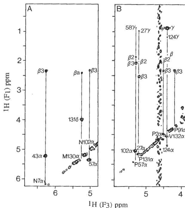
Fig. 5. Two ^1\text{H}(\text{F}_1) - ^1\text{H}(\text{F}_3) planes at different ^{13}\text{C} frequencies of the 3D ^{13}\text{C} -separated ROESY-HMQC spectrum of ^{13}\text{C}/^{15}\text{N} labeled IL-1 \beta recorded with a 22 ms mixing time. (A) ROEs to the \text{C}^\alpha\text{H} protons of Asn-7, Asn-102 and Met-130 at \delta^{13}\text{C} = 51.4 (\pm \text{nSW}) ppm (the spectral width SW is 20.71 ppm). Only positive levels are shown and diagonal resonances are therefore not observed. In the case of Asn-7 and Asn-102, \chi_1 \sim -60^\circ , while for Met-130 we were unable to make the distinction between \chi_1 \sim -60^\circ and \chi_1 \sim 180^\circ . Note, however, that for Met-130, a ROE between the \text{C}^\alpha\text{H} proton and only one of the two \text{C}^\beta\text{H} protons, namely the low-field \text{C}^\beta\text{H} , is observed, indicative of an ordered conformation with \chi_1 \sim -60^\circ or -180^\circ . (B) ROEs to the \text{C}^\alpha\text{H} protons of Pro-2, Pro-57, Pro-91, Pro-131 and Val-132 at \delta^{13}\text{C} = 61.9 (\pm \text{nSW}) ppm. Note that in addition to intraresidue ROEs, a number of both short and long range interresidue ROEs are observed in both slices. The assignments are from Clare et al. (1990c).
