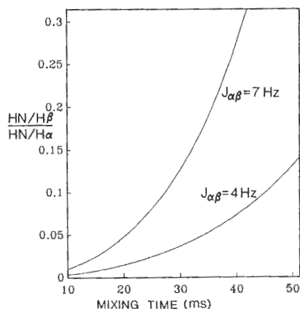
Fig. 3. Ratio of the HN-C H and HN-C β H cross-peak intensities when both C β H methylene protons have identical couplings to the C α H proton. The HN-C β H cross-peak intensity corresponds to a single C β H proton (i.e. if the two C β H protons have degenerate chemical shifts the cross-peak ratio will be twice that shown in the graph). The cross-peak ratios have been calculated with ^3J_{\text{HN}\alpha} = 7 Hz and no C γ H protons.
