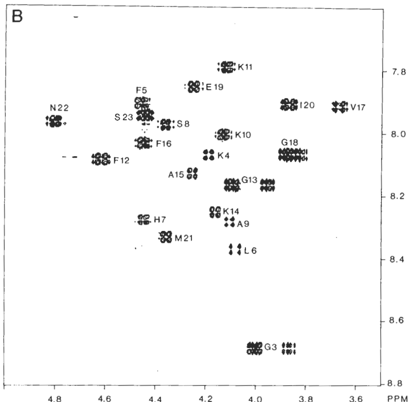
Figure 3 (A) 600 MHz COSY spectrum of 12 mg magainin 2 in 0.5 ml 75% \text{H}_2\text{O}/25\% trifluoroethanol- \text{d}_3 . The drawn lines in (A) identify the coupled protons of Val-17. \text{CaH-CH}_3 cross peaks of the two alanine residues are marked Ala. The boxed region (commonly known as the "fingerprint region") shows interactions between NH and \text{CaH} protons and is enlarged in (B). In this enlargement a single cross multiplet, consisting of a number of closely spaced multiplet components, is observed for each nonglycine amino acid with the exception of the two N-terminal residues, for which the NH protons exchange rapidly with the solvent. For glycine residues, two cross peaks are observed corresponding to the two nonequivalent \text{CaH} protons. For Gly-18, the chemical shifts of the two \text{CaH} protons differ by only 0.04 ppm, and the two multiplets nearly overlap. For both Gly-3 and Gly-13 the \text{CaH} chemical shifts differ by about 0.2 ppm, and the label is positioned in between the two cross peaks.
