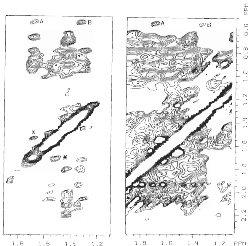
Figure 10 Comparison of small regions of the NOESY spectra of [ ^{13}\text{C} ]Ala lambda repressor. The left panel shows the result of NOE editing and exhibits interactions only to ^{13}\text{C} -labeled protons, i.e. to the alanine methyl groups. The right panel shows the identical region of the conventional NOESY spectrum. Both spectra were recorded with a 300 ms NOE mixing time. From Bax & Weiss (149). Reprinted with permission from the Journal of Magnetic Resonance . Copyright 1987, Academic.
