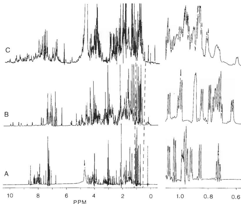
Figure 1 ^1\text{H} NMR spectra of (A) magainin 2 (23 amino acids) in 75% \text{H}_2\text{O} , 25% trifluoroethanol- \text{d}_3 , (B) basic pancreatic trypsin inhibitor (58 amino acids) in ^2\text{H}_2\text{O} , and (C) staphylococcal nuclease (156 amino acids) in 90% \text{H}_2\text{O} /10% ^2\text{H}_2\text{O} . All spectra were recorded at 27^\circ\text{C} at 600 MHz and identical digital filtering was used for all three spectra to sharpen the individual resonances. Note that because of hydrogen exchange most but not all amide protons are replaced by deuterons in the BPTI spectrum. In the expansions of the regions between the broken lines, shown on the right, J splittings of the resonances are observed.
