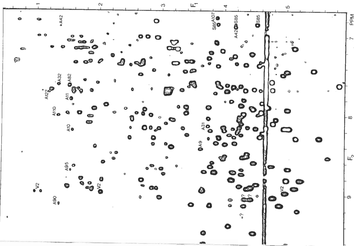
G. 7. Two-dimensional HOHAHA spectrum of hen egg white lysozyme, 4.5 mM, pH 5 mM NaCl, 35°. The spectrum was recorded with the scheme of Fig. 6, using a mixing of 35 msec, 24- \mu sec 90° pulse width, 800 \times 2048 data matrix, acquisition times of 40 and 160 msec in t_1 and t_2 dimension, respectively. Sixteen scans were recorded per t_1 value and total measuring time was 7 hr. Assignments are taken from Redfield and Dobson. 31 No baseline correction procedure of the frequency domain spectra was used and the lowest
