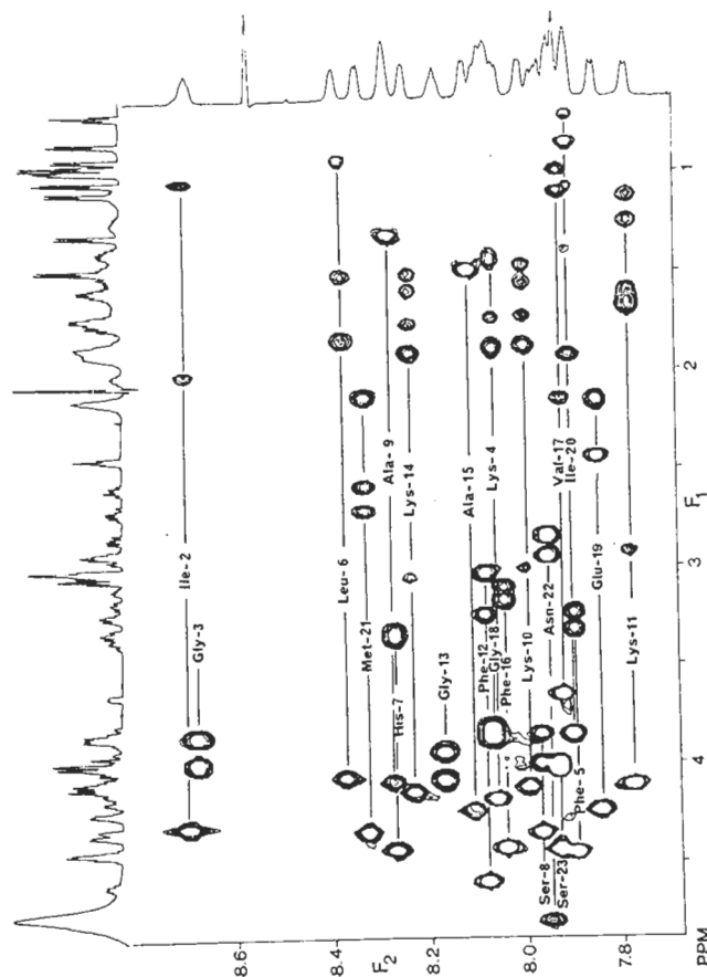
FIG. 4. Expansion of the boxed region of Fig. 3, showing the amide to side-chain connectivities. With the exceptions of Gly-1 and Ile-2, for each amide proton nearly all side-chain resonances connected directly or indirectly via scalar couplings to the \text{C}_\alpha\text{-H} resonance are observed, despite relatively small \text{NH-C}_\alpha\text{H} J couplings ( \alpha helix).
