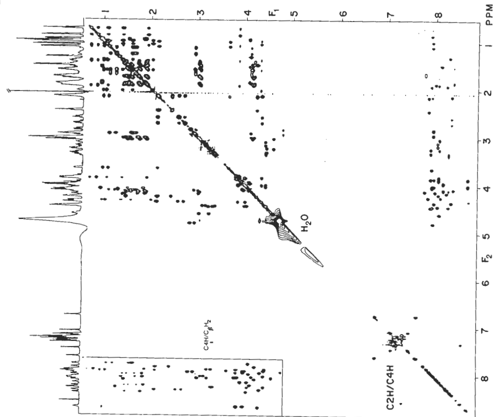
FIG. 3. Two-dimensional HOHAHA spectrum of the peptide magainin 2, 15 mg in 0.375 ml \text{H}_2\text{O}/0.125 ml trifluoroethanol, 27^\circ . The spectrum was recorded at 600 MHz, using a WALTZ17 mixing sequence with \alpha = 60^\circ . The 90^\circ pulse width was 35 \mu\text{sec} , duration of the WALTZ irradiation was 75 msec, and the trim pulse duration was 2 msec. Presaturation of the \text{H}_2\text{O} resonance was used during the recycling delay. Data were acquired in the TPPI mode and the size of the acquired data matrix was 700 \times 2048 , corresponding to acquisition times of 42 and 120 msec in the t_1 and t_2 dimension, respectively. Eight scans, preceded by two dummy scans, were recorded per t_1 value, and the total measuring time was 3.5 hr. Zero filling was used to yield a digital resolution of 4 Hz in both dimensions.
