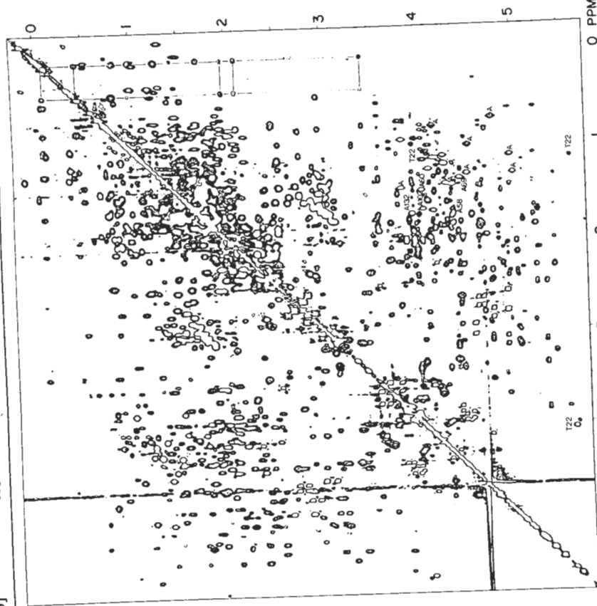
Fig. 5. Two-dimensional HOHAHA spectrum of the aliphatic region of a staphylococcal nuclease/pdTp/ Ca^{2+} complex (18 kDa), 1.5 mM in D_2O , 100 mM NaCl, pH 7.4. The spectrum was recorded with a mixing time of 35 msec and the measuring time was 6 hr. Duration of the trim pulses was 1.5 msec and the 90^\circ pulse width was 28 \mu sec. Labeled cross-peaks follow the assignments of Torchia et al. 28
